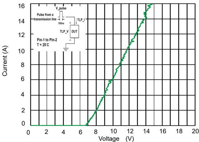
Fig 5. TLP Measurement
