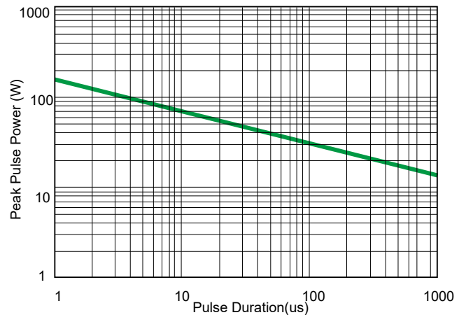
Fig 6. Non Repetitive Peak Pulse Power vs. Pulse time
