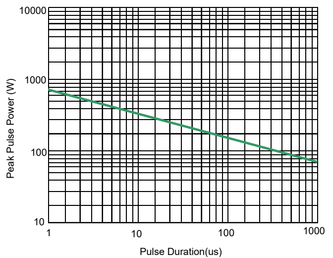
Fig 6. Non-Repertive Peak Pulse Power vs. Pulse time
