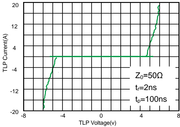
Fig 3. TLP Measurement
