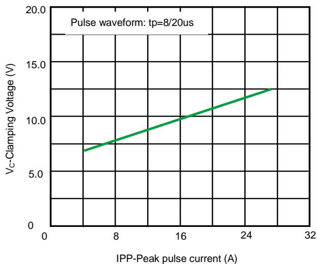
Fig 5. Clamping voltage vs. Peak pulse current
